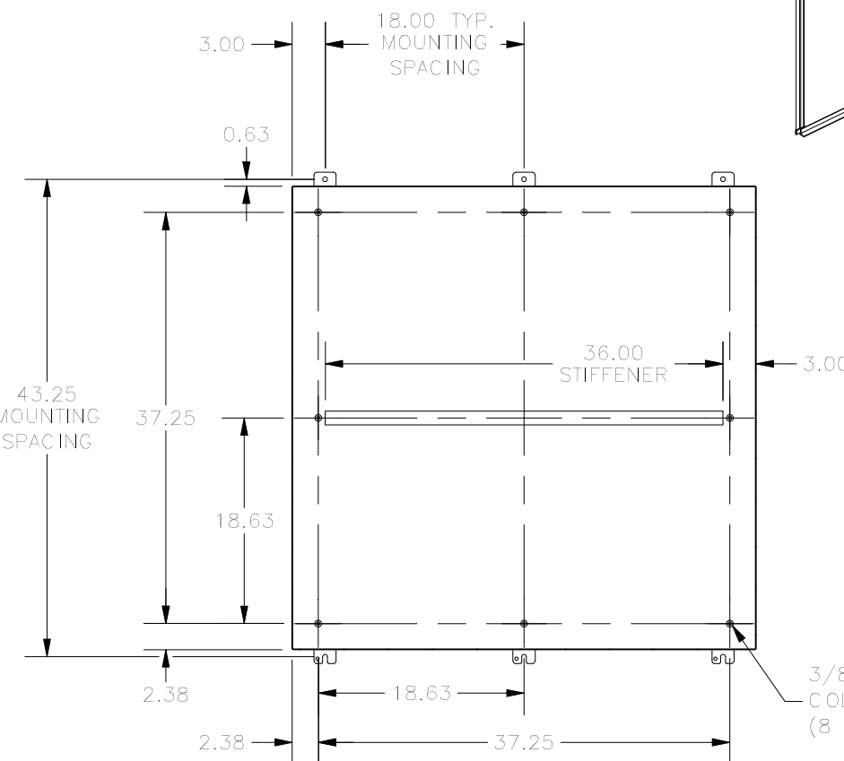
SECTION A-A (INSIDE BACK VIEW OF ENCL.)
