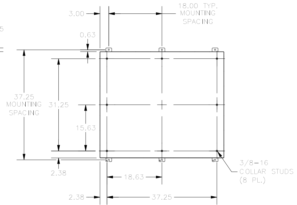
SECTION A-A (INSIDE BACK VIEW OF ENCL.)
