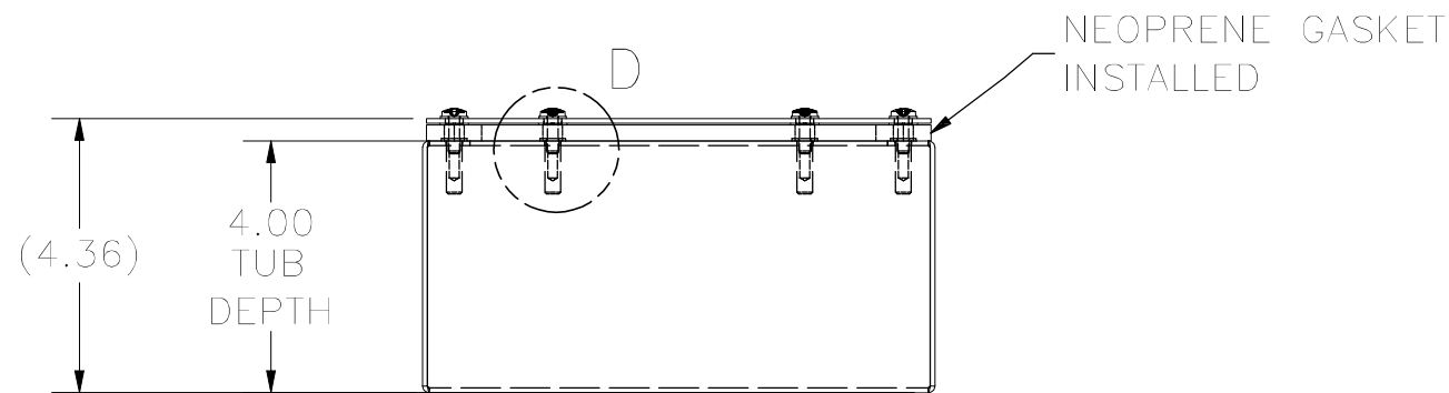
BOTTOM VIEW
