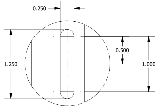
DETAIL A (30 PL.) (SLOT DETAIL)
