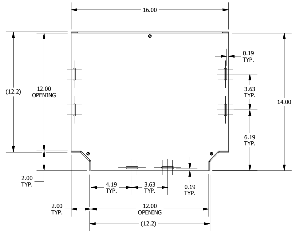
TOP VIEW
