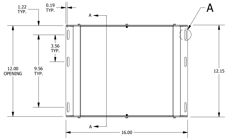
FRONT VIEW
