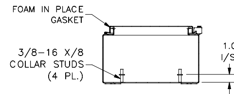
SECTION B-B (INSIDE TOP OF ENCL.)
