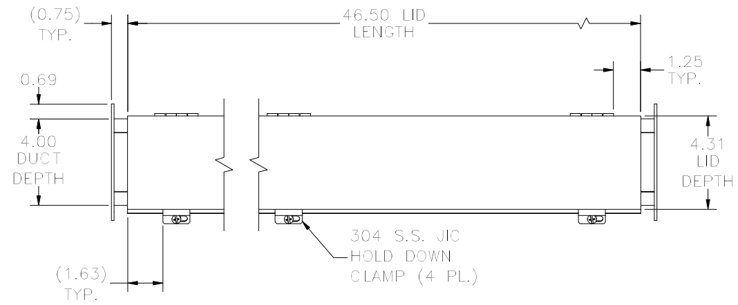
TOP VIEW
