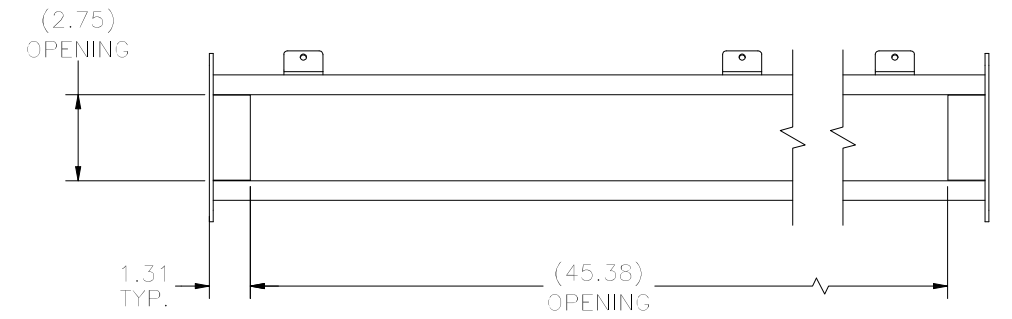
TOP VIEW (LID ASSM. NOT SHOWN)
