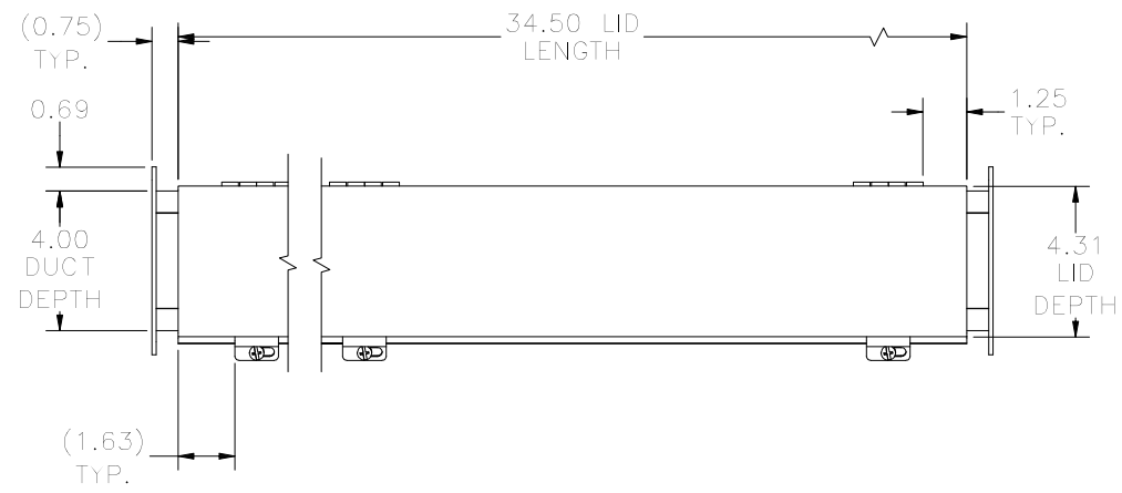
TOP VIEW
