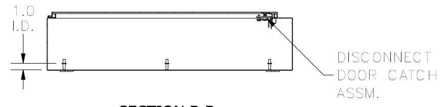
SECTION B-B (INSIDE TOP OF ENCLOSURE)
