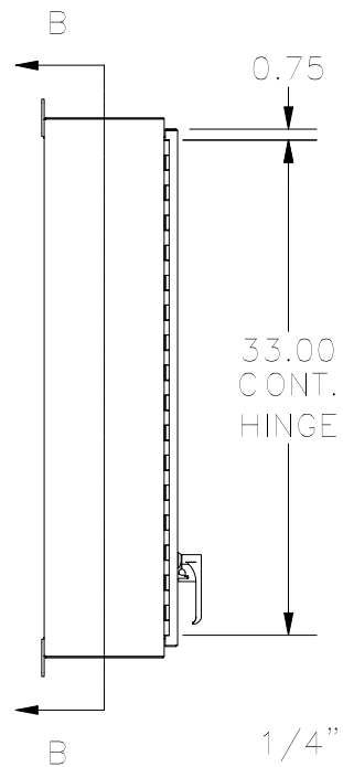
LEFT VIEW
