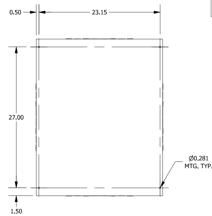
BACK VIEW
