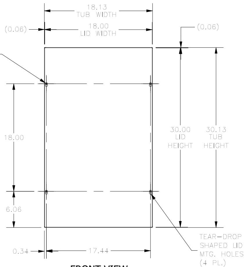
FRONT VIEW
