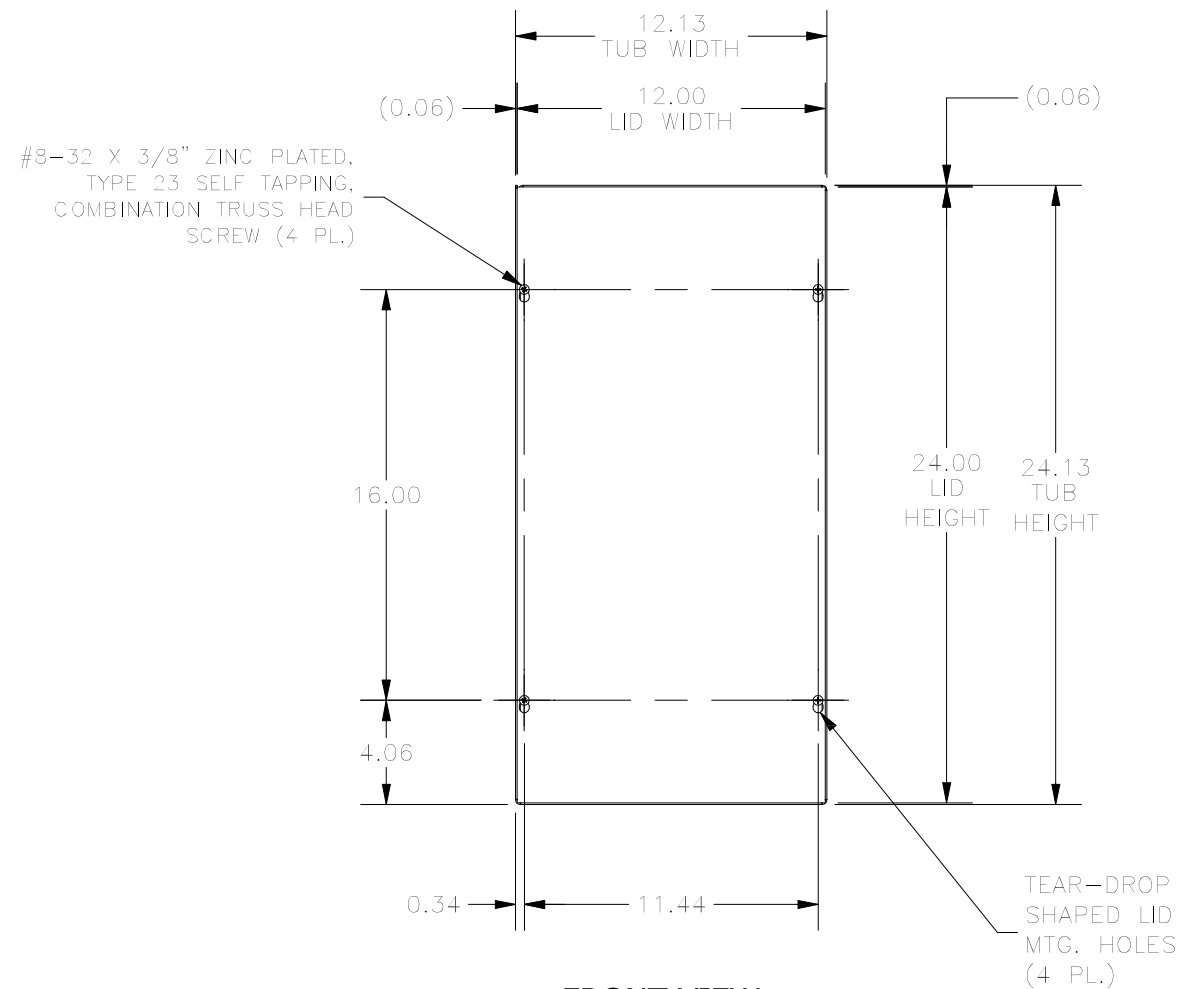
FRONT VIEW
