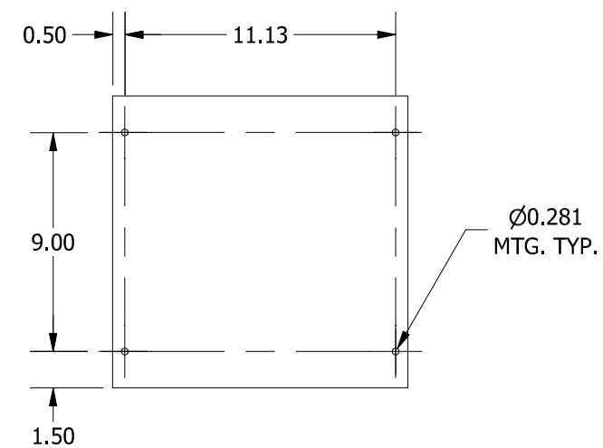
BACK VIEW
