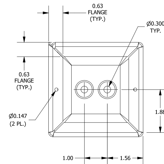
FRONT VIEW LID REMOVED
