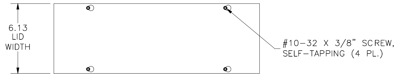
TOP VIEW
