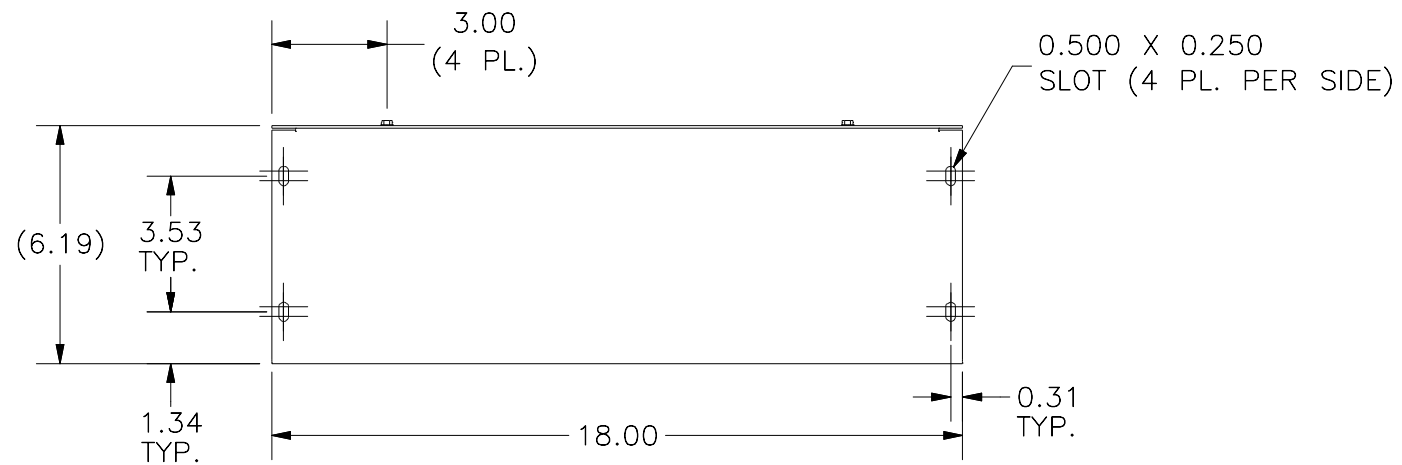
FRONT VIEW
