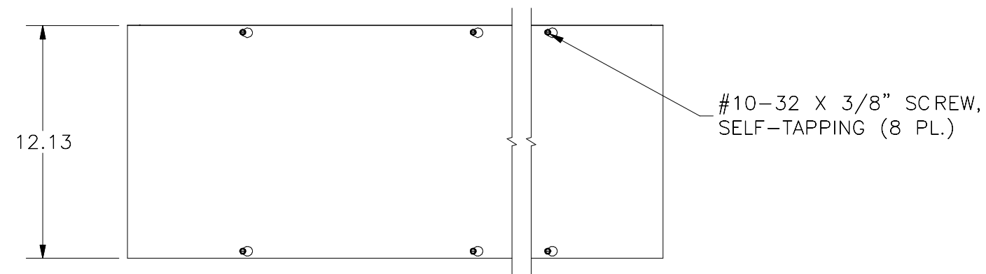
TOP VIEW
