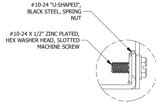
DETAIL A (5 PL.) (LID ATTACHMENT DETAIL)
