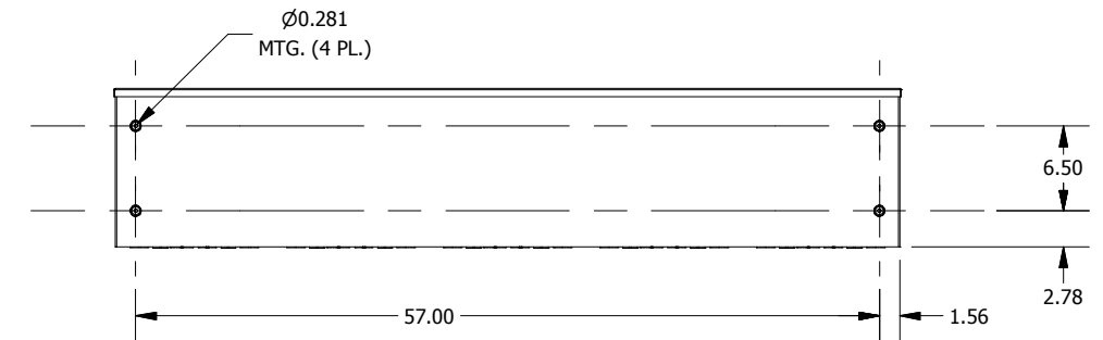
BACK VIEW
