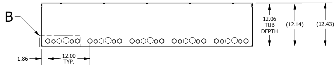
BOTTOM VIEW
