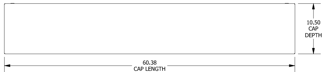
TOP VIEW
