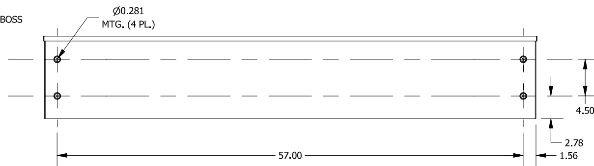
BACK VIEW
