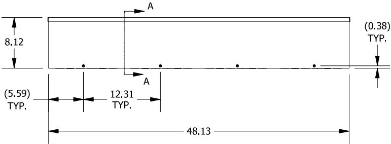
FRONT VIEW
