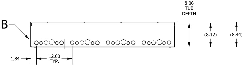
BOTTOM VIEW
