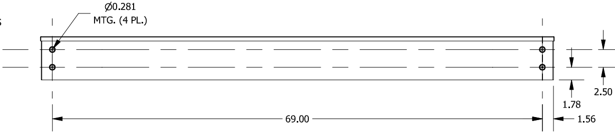
BACK VIEW
