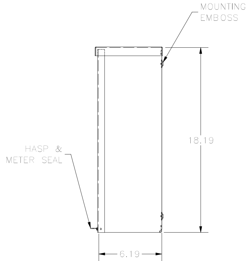
RIGHT VIEW
