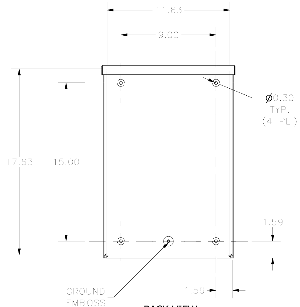
BACK VIEW
