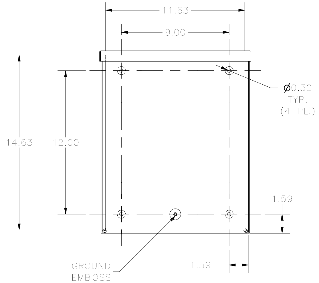
BACK VIEW
