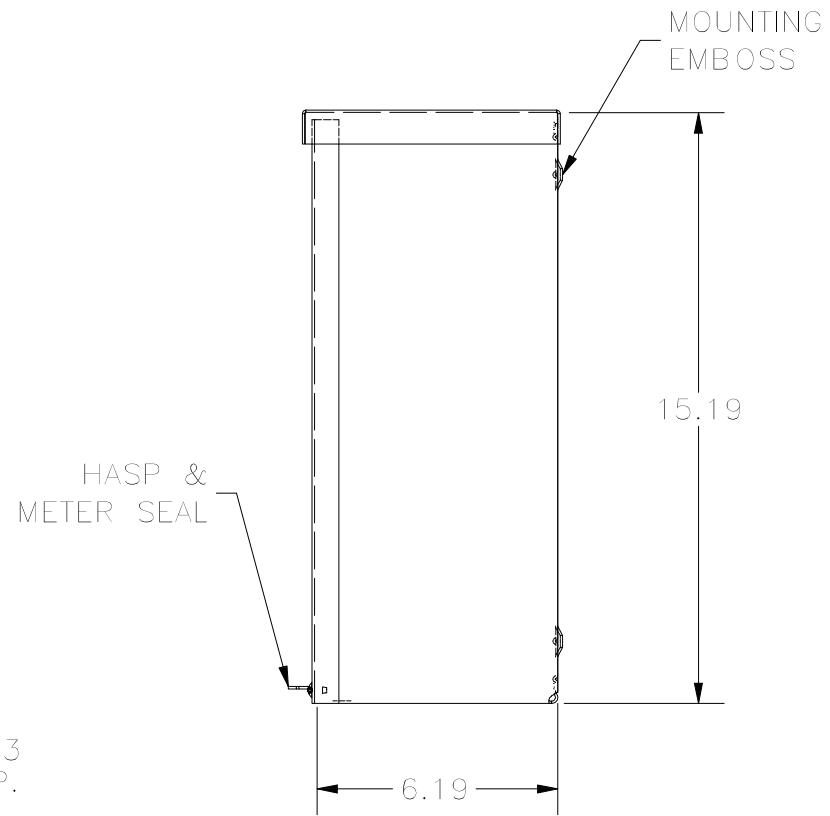
RIGHT VIEW
