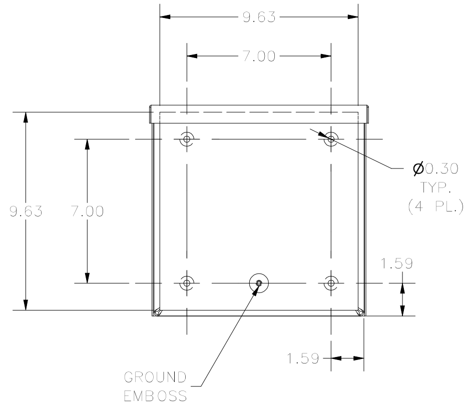
BACK VIEW
