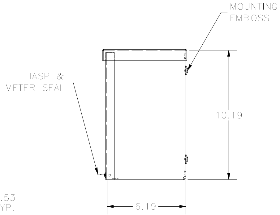
RIGHT VIEW
