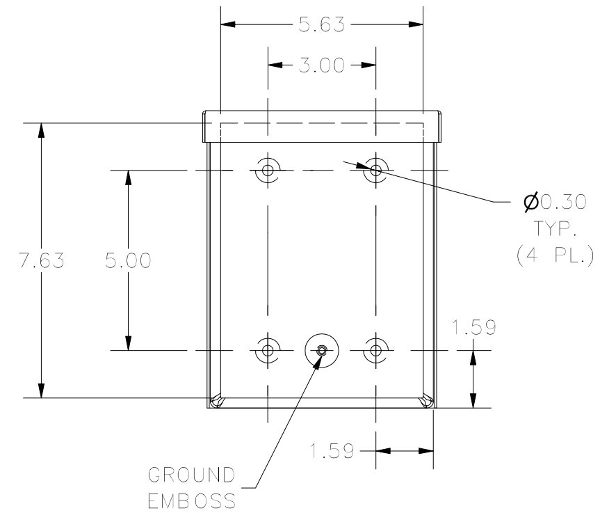
BACK VIEW
