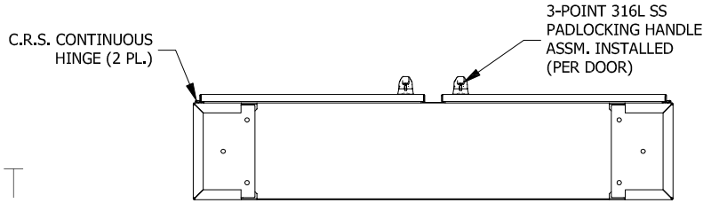
BOTTOM VIEW
