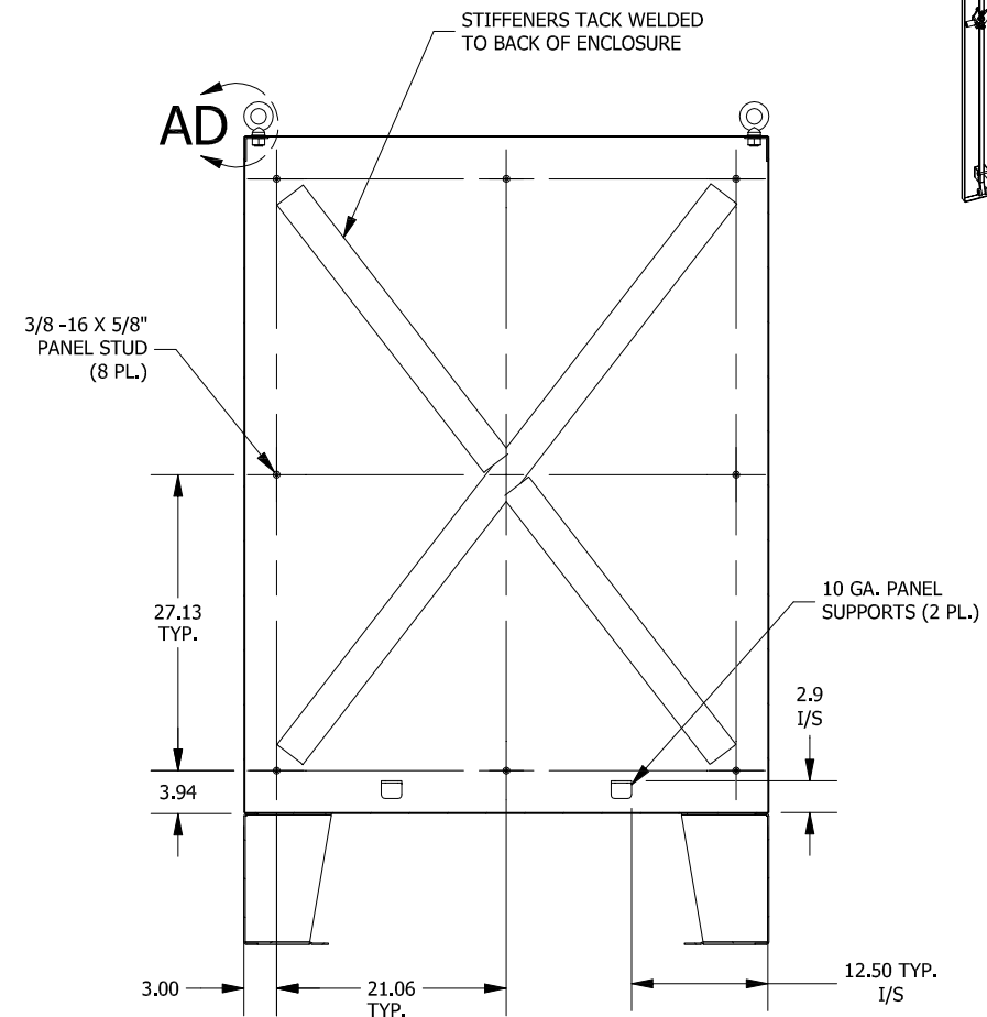
SECTION A-A (INSIDE BACK VIEW OF ENCLOSURE)
