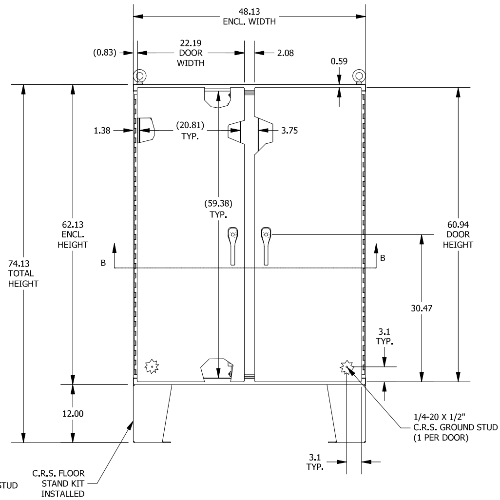
FRONT VIEW
