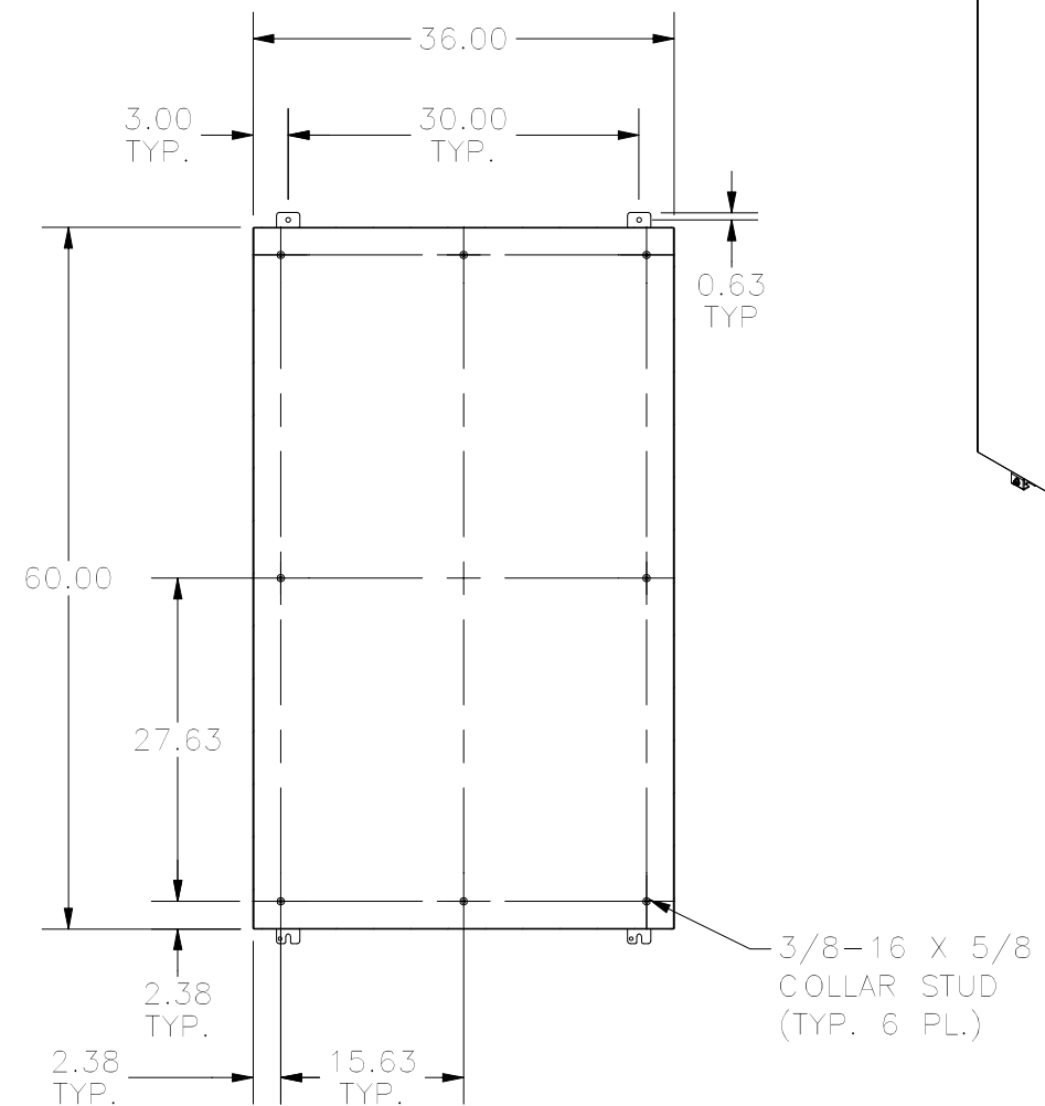
SECTION A-A (INSIDE BACK OF TUB)
