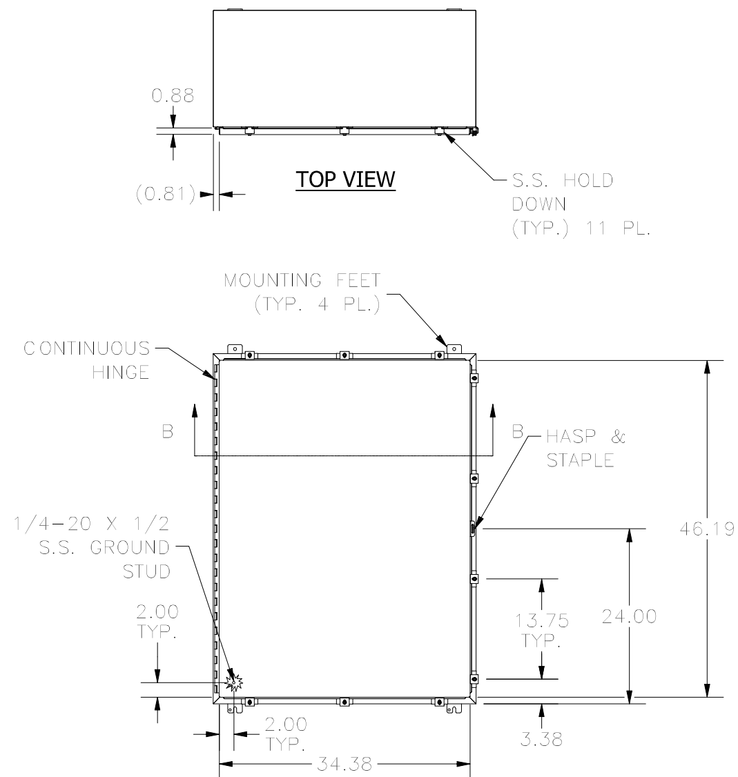
FRONT VIEW
