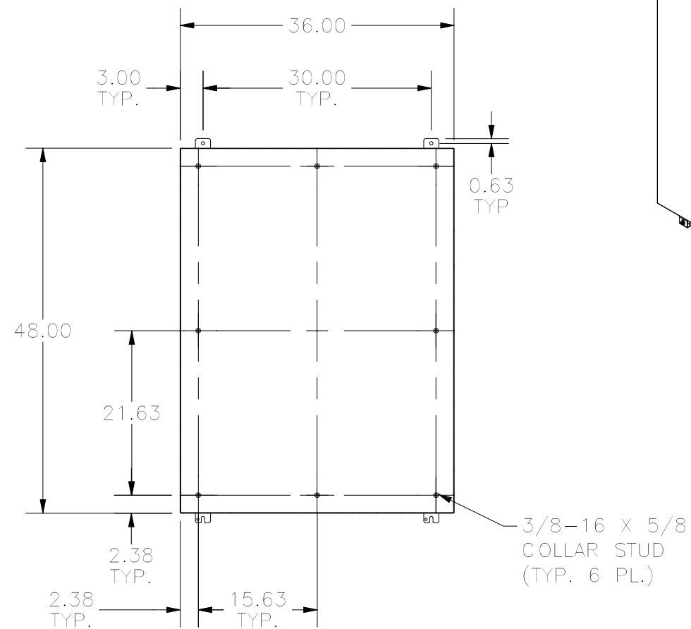
SECTION A-A (INSIDE BACK OF TUB)
