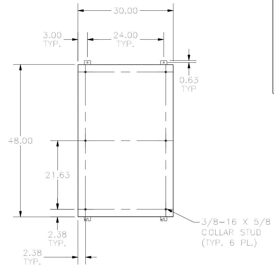
SECTION A-A (INSIDE BACK OF TUB)
