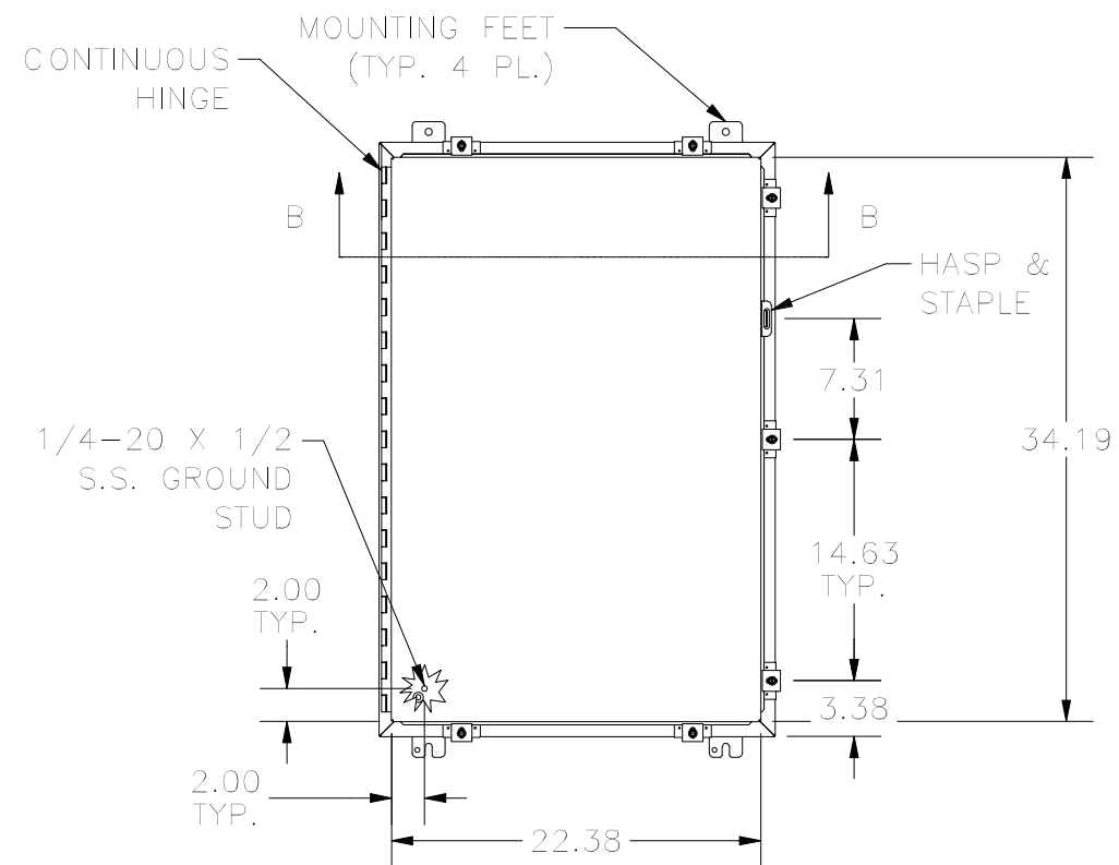
FRONT VIEW
