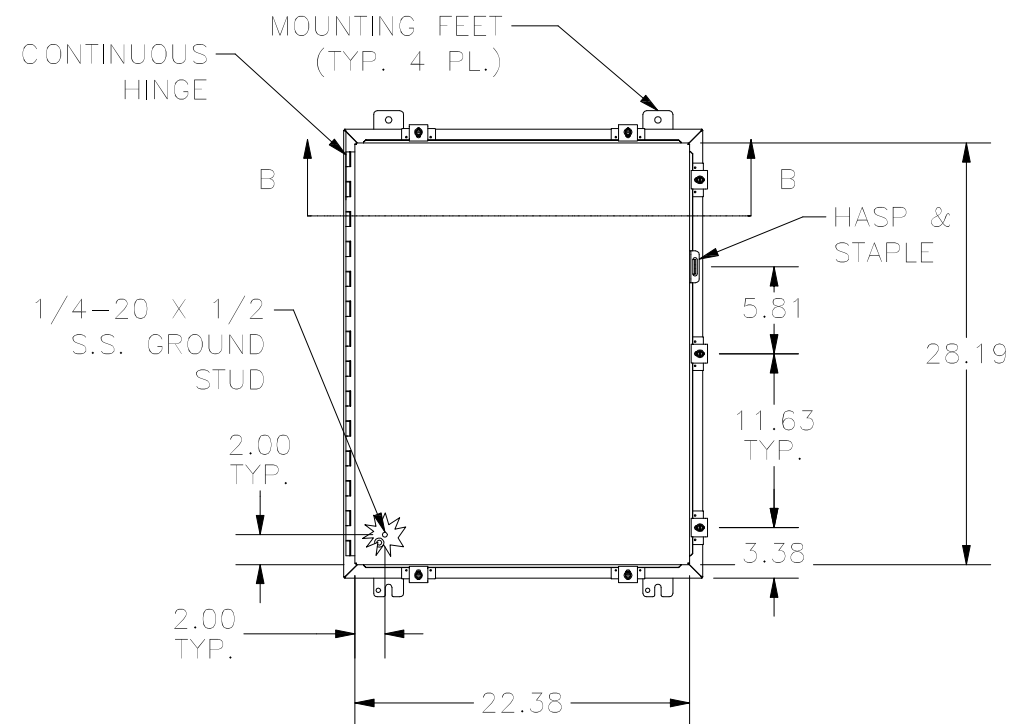
FRONT VIEW
