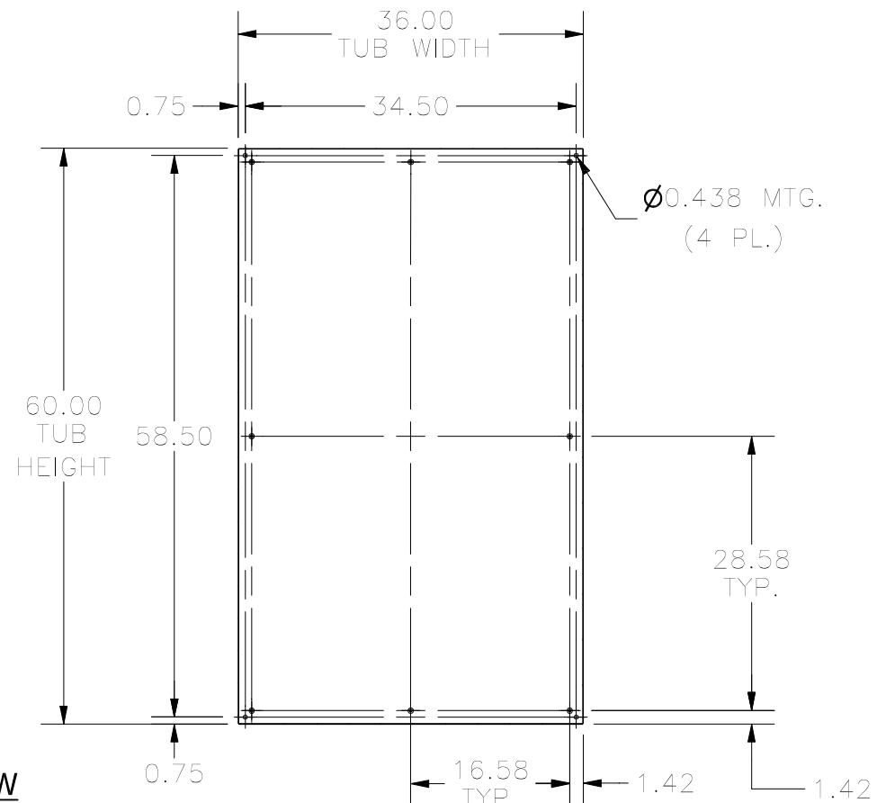
SECTION Y-Y (INSIDE BACK OF ENCLOSURE)
