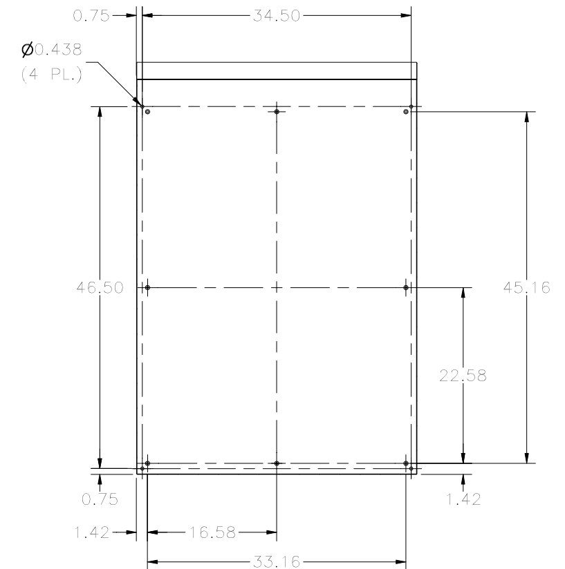
SECTION A-A VIEW (INSIDE BACK OF ENCL.)
