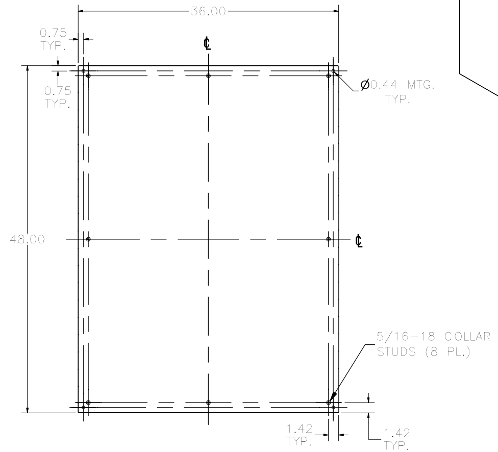
SECTION E-E VIEW (INSIDE BACK OF ENCLOSURE)
