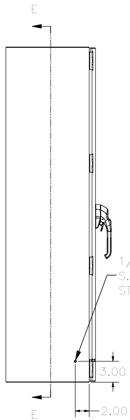
LEFT SIDE VIEW
