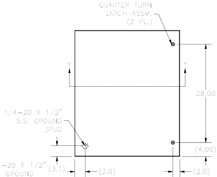
FRONT VIEW
