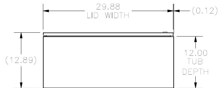
BOTTOM VIEW
