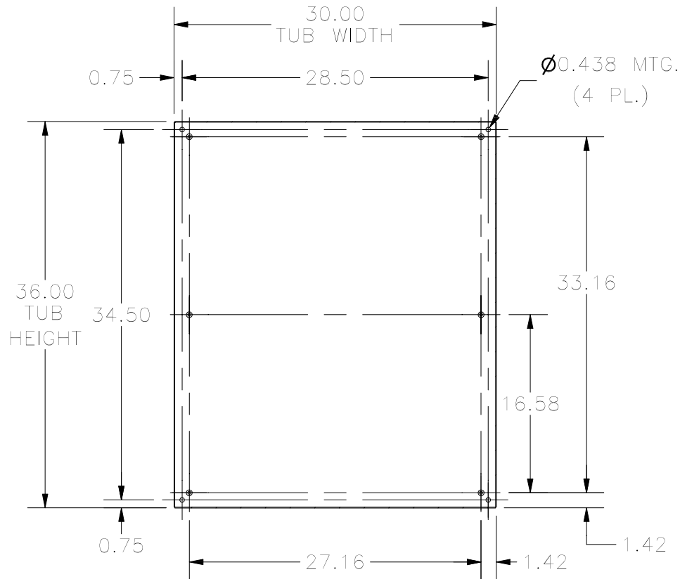
SECTION W-W (INSIDE BACK OF ENCLOSURE)
