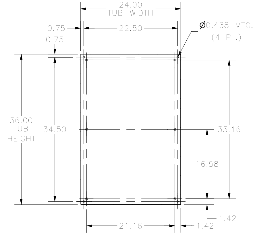
SECTION W-W (INSIDE BACK OF ENCLOSURE)
