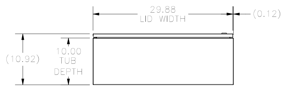
BOTTOM VIEW
