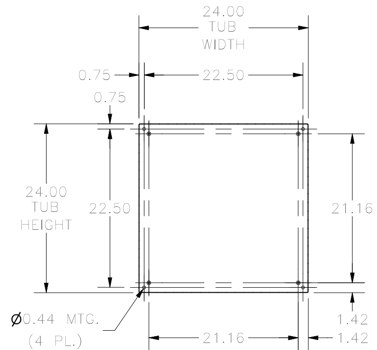
SECTION Y-Y (INSIDE BACK OF ENCLOSURE)
