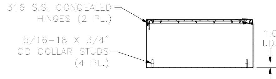
SECTION AA-AA (INSIDE TOP OF ENCLOSURE)
