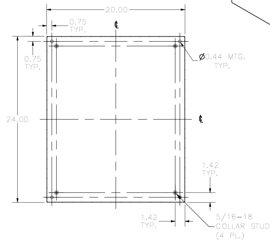
SECTION D-D VIEW (INSIDE BACK OF ENCLOSURE)
