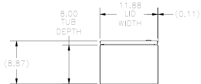
BOTTOM VIEW
