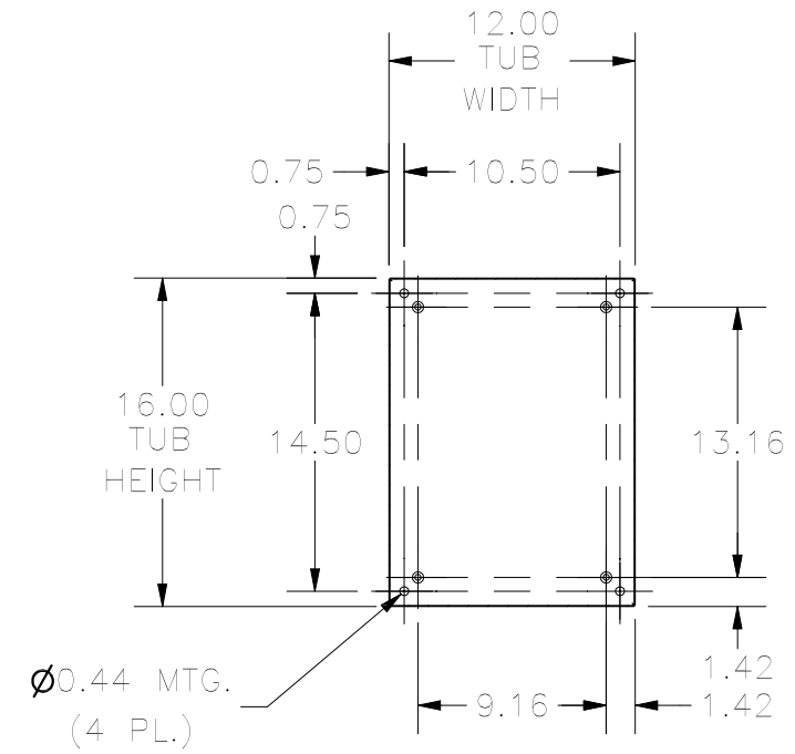
SECTION Y-Y (INSIDE BACK OF ENCLOSURE)
