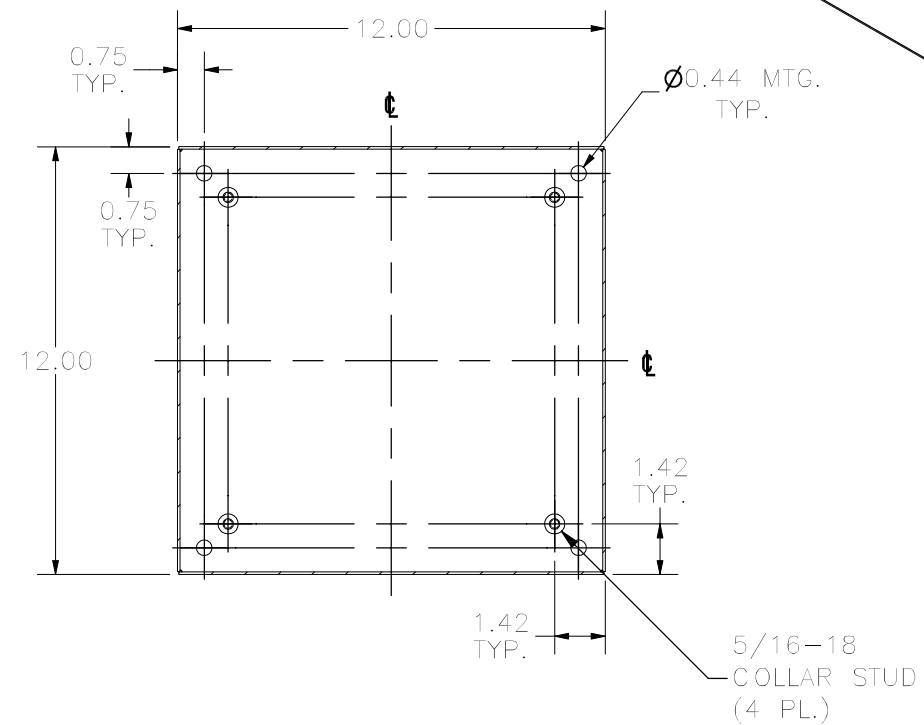
SECTION D-D VIEW (INSIDE BACK OF ENCLOSURE)
