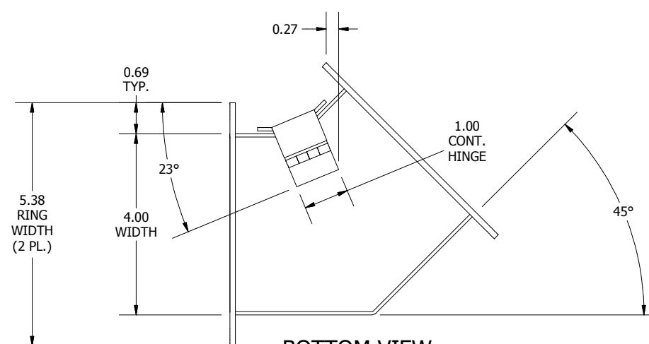
BOTTOM VIEW
