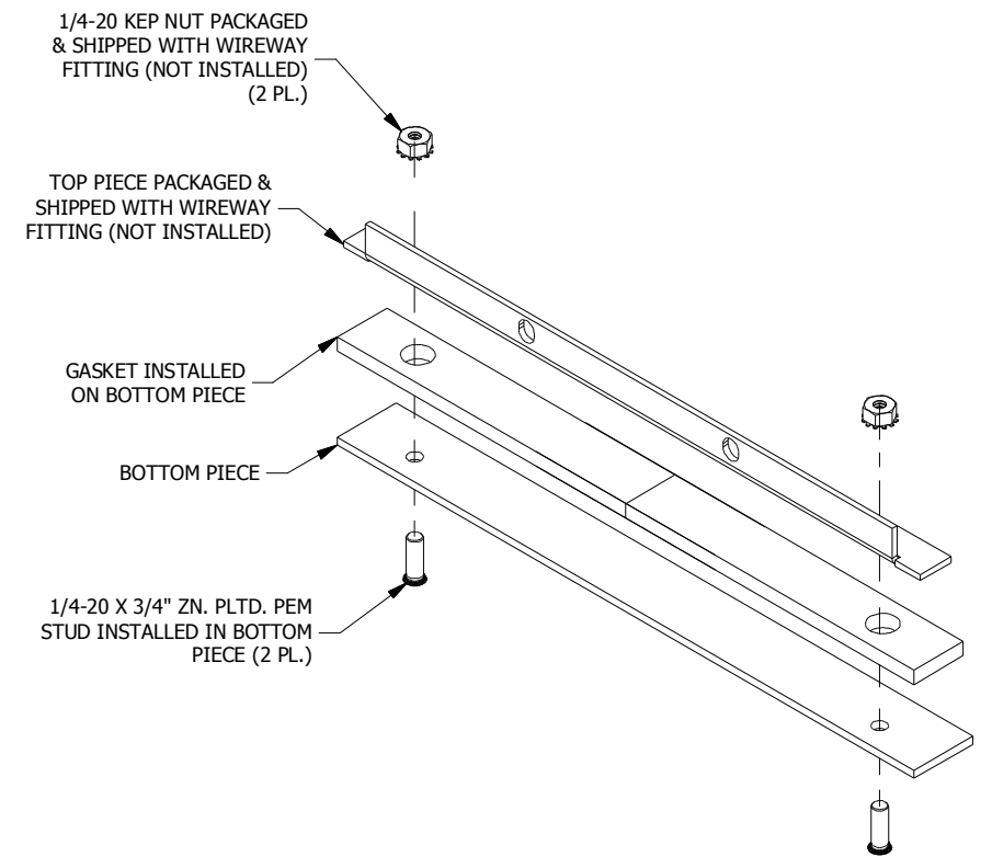
ASSEMBLY EXPLODED VIEW
