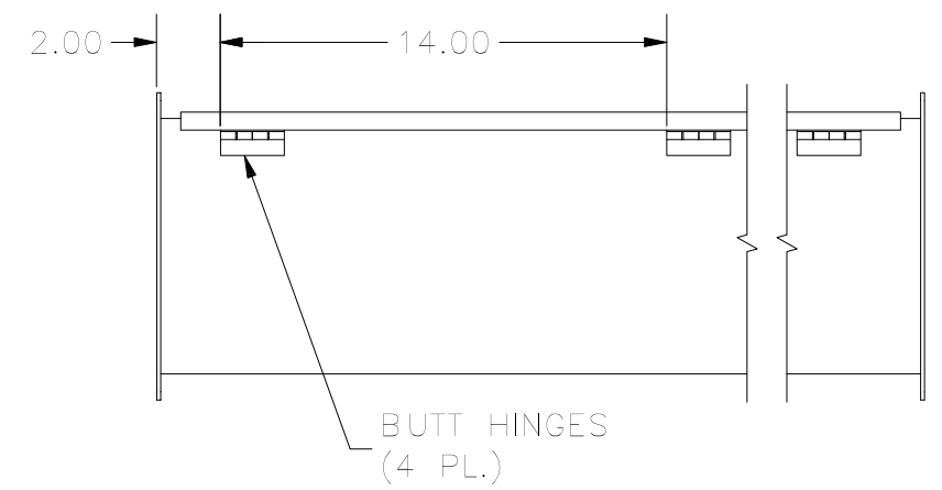
BACK VIEW
