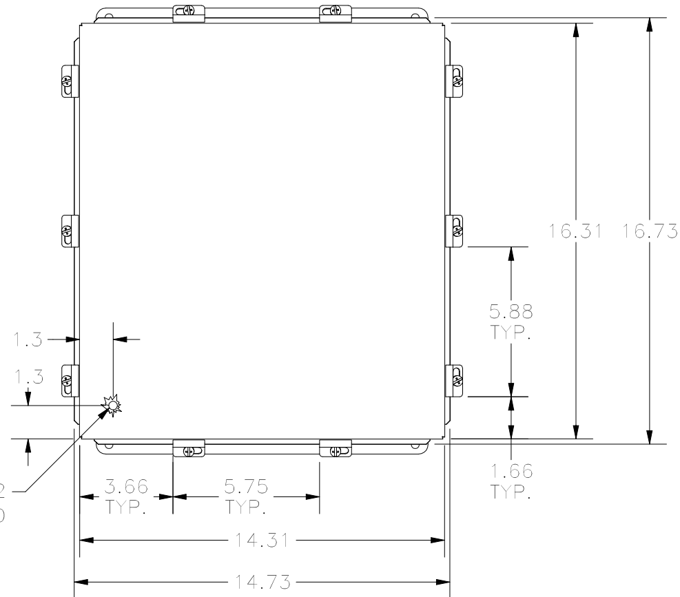
FRONT VIEW
