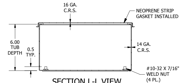
SECTION L-L VIEW (INSIDE TOP OF ENCL.)
