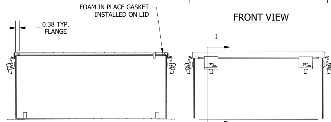
SECTION J-J
