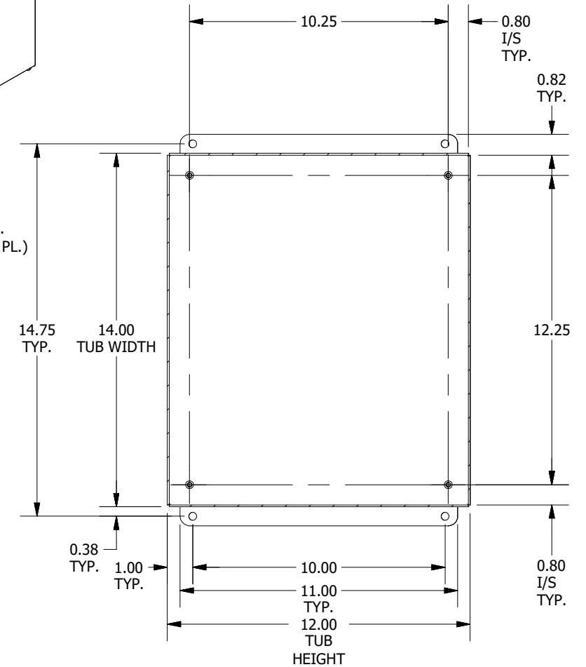
SECTION F-F (INSIDE BACK VIEW)
