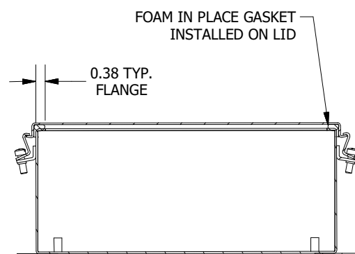
SECTION J-J
